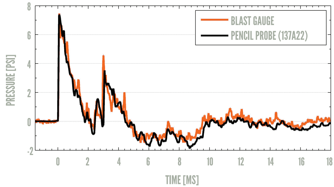
ACCURATE CAPTURE OF BLAST OVERPRESSURE: BLAST GAUGE SYSTEM VS. PENCIL PROBE
